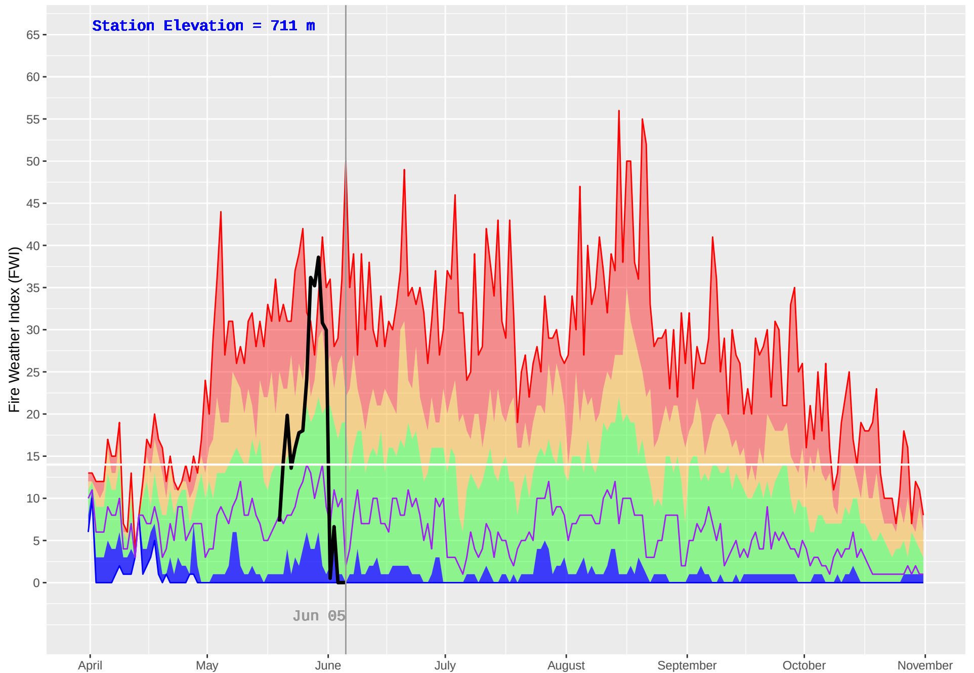
TOAD RIVER (126) : Historical (1981–2018) and Current (2019) Daily Fire Weather Index (FWI)
