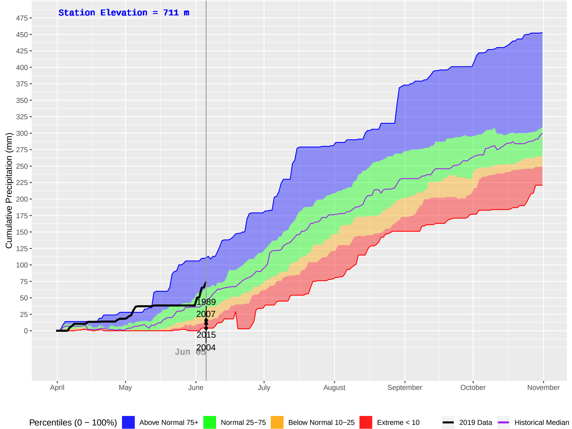
TOAD RIVER (126) : Historical (1981–2018), Current (2019) Daily Cumulative Precipitation
