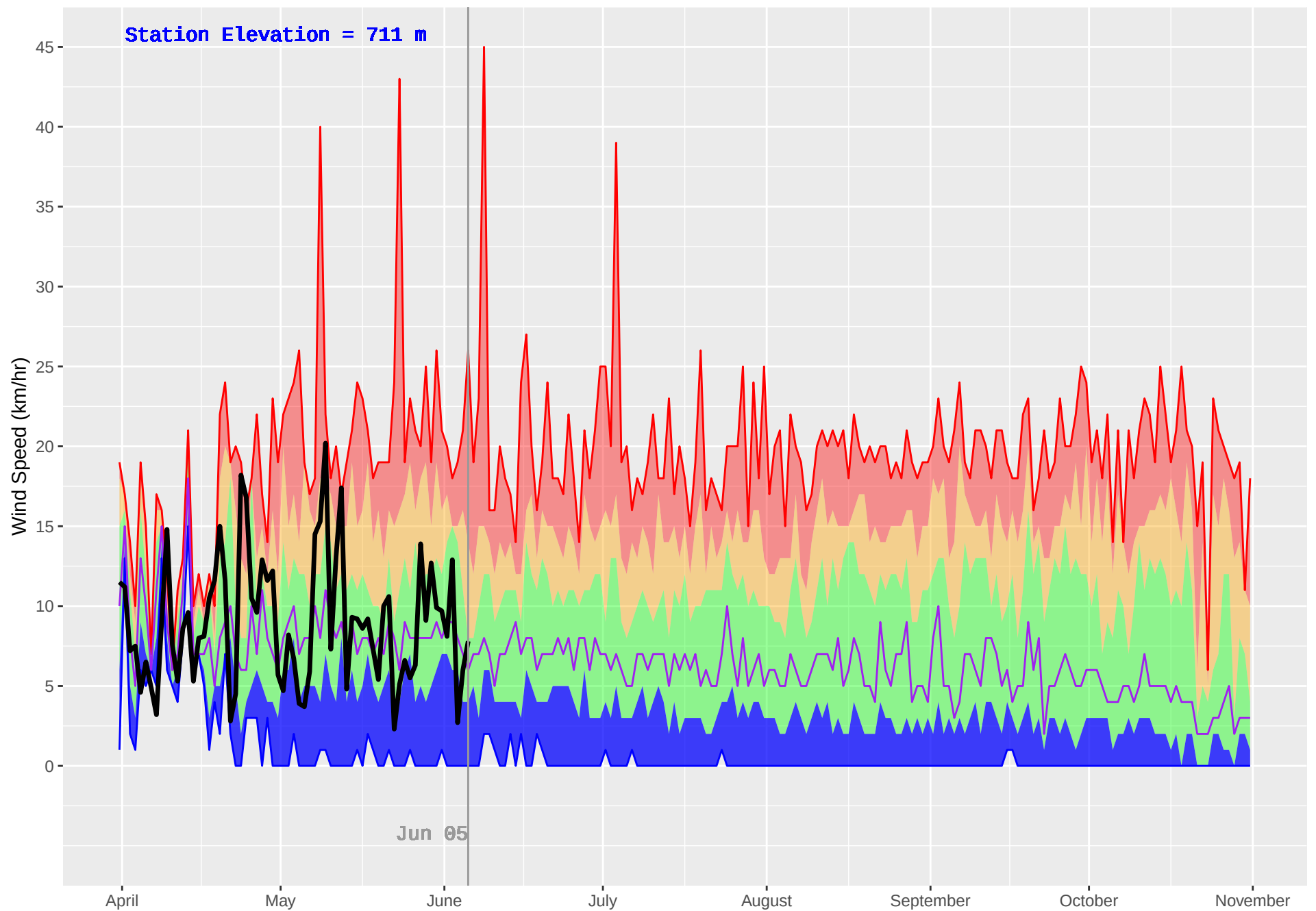
TOAD RIVER (126) : Historical (1981–2018) and Current (2019) Daily Wind Speed
