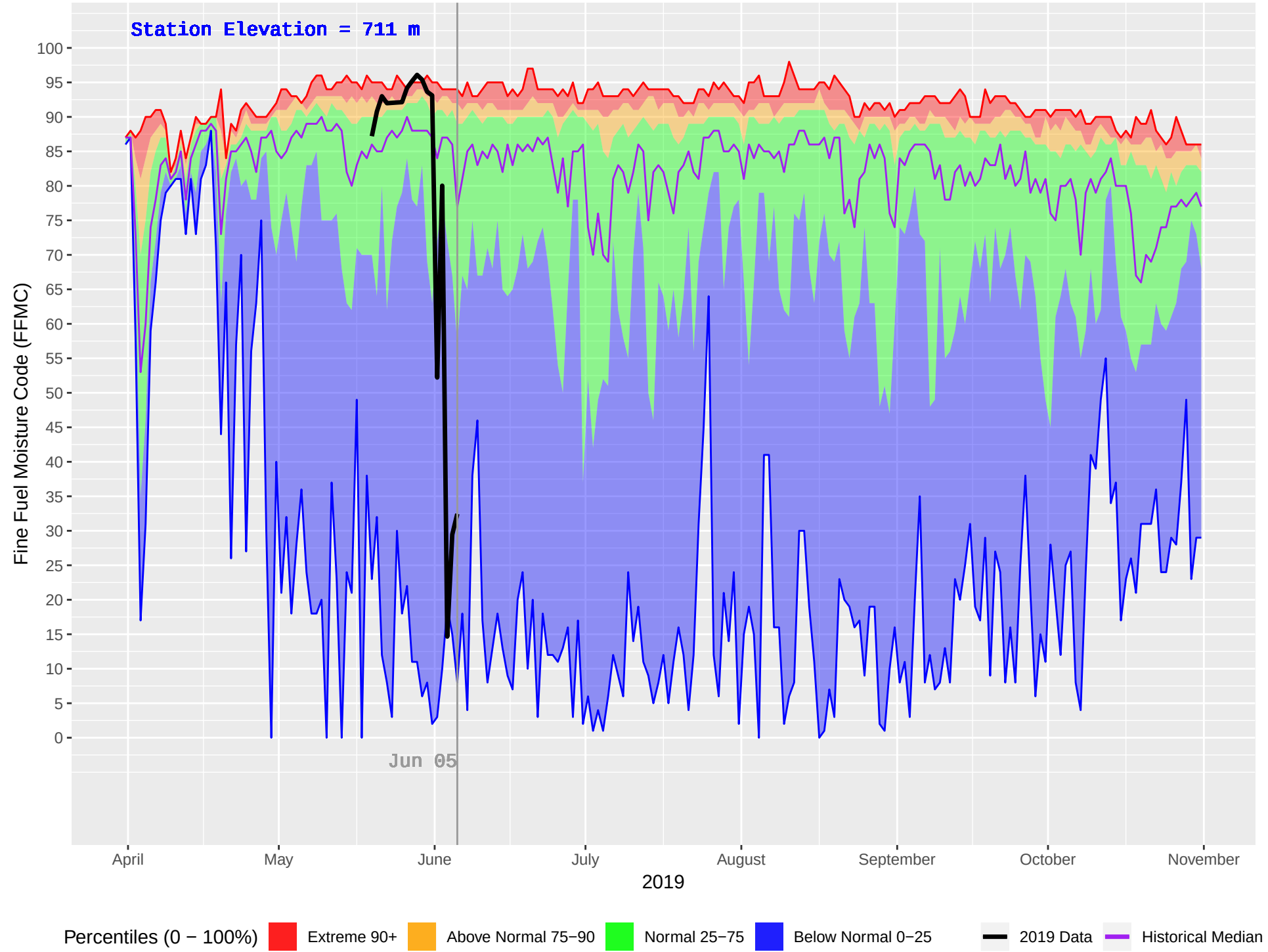
TOAD RIVER (126) : Historical (1981–2018) and Current (2019) Daily Fine Fuel Moisture Code (FFMC)
