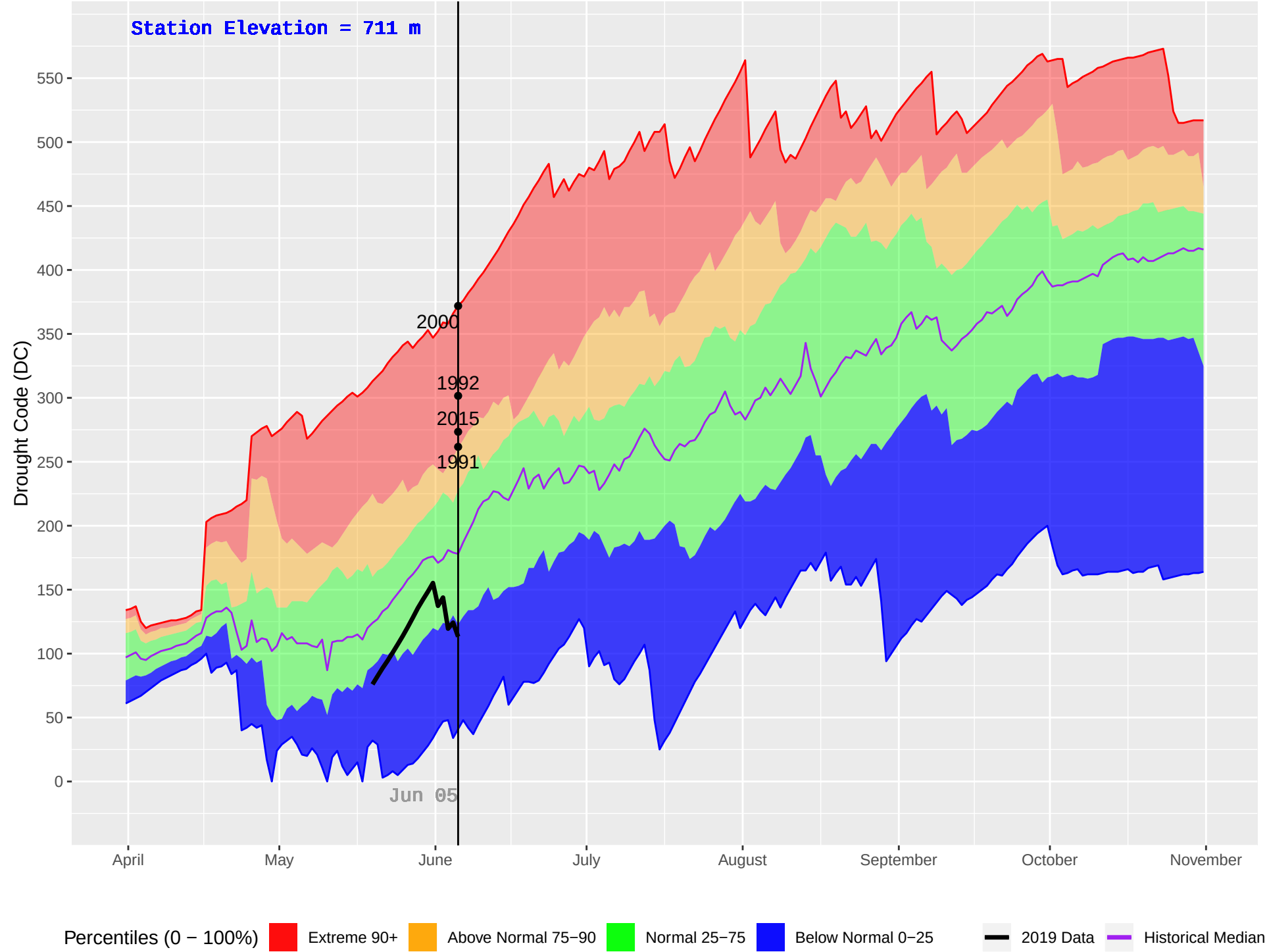
TOAD RIVER (126) : Historical (1981–2018) and Current (2019) Daily Drought Code (DC)
