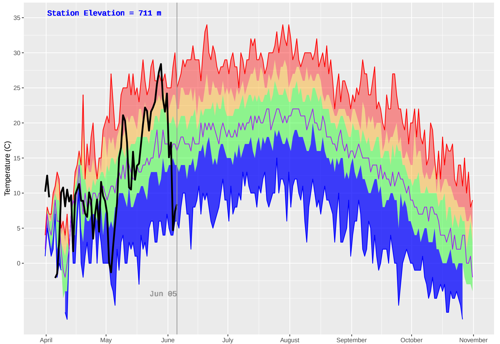
TOAD RIVER (126) : Historical (1981–2018) and Current (2019) Daily Temperature
