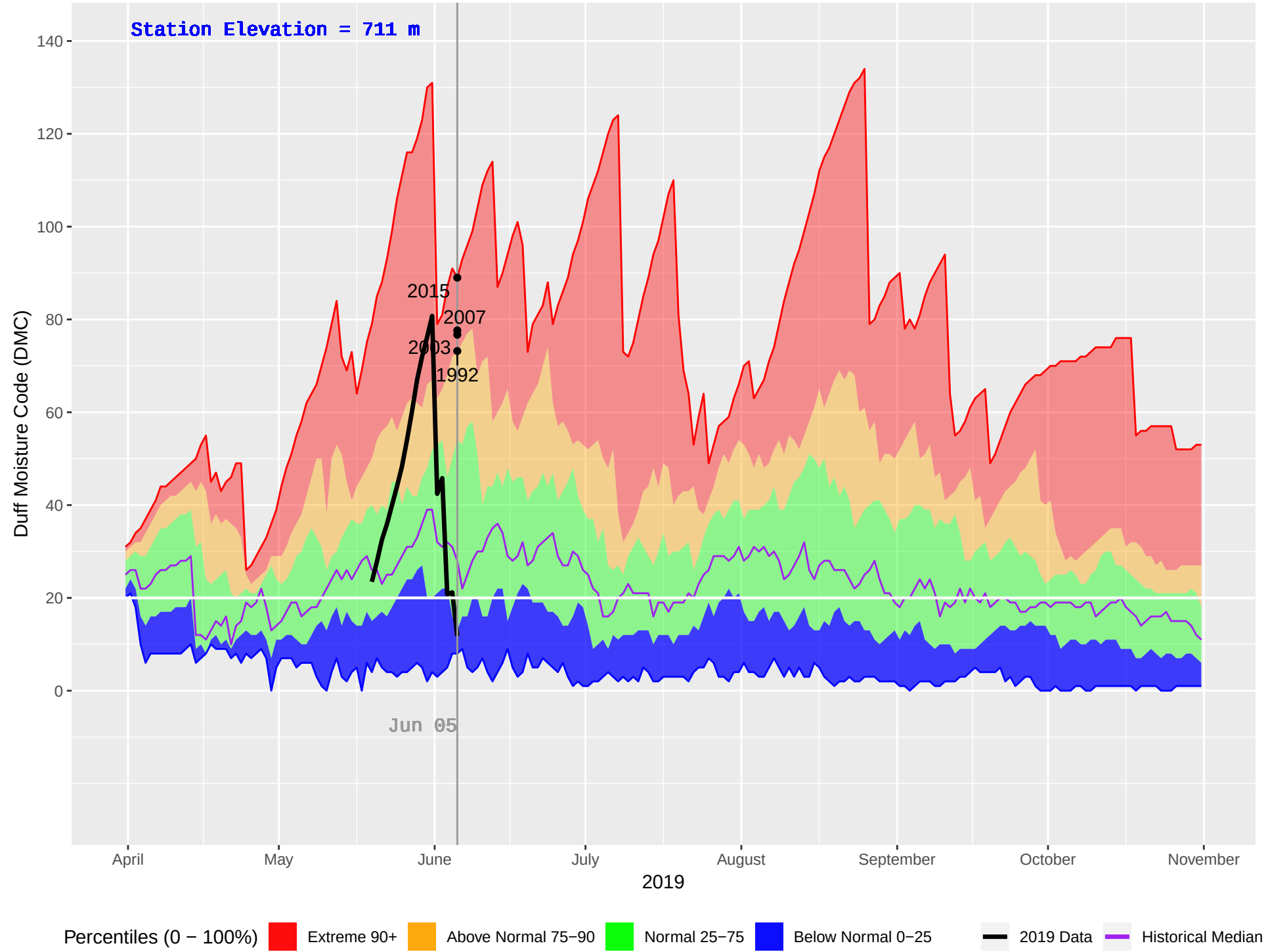
TOAD RIVER (126) : Historical (1981–2018), Current (2019) Daily Duff Moisture Code (DMC)
