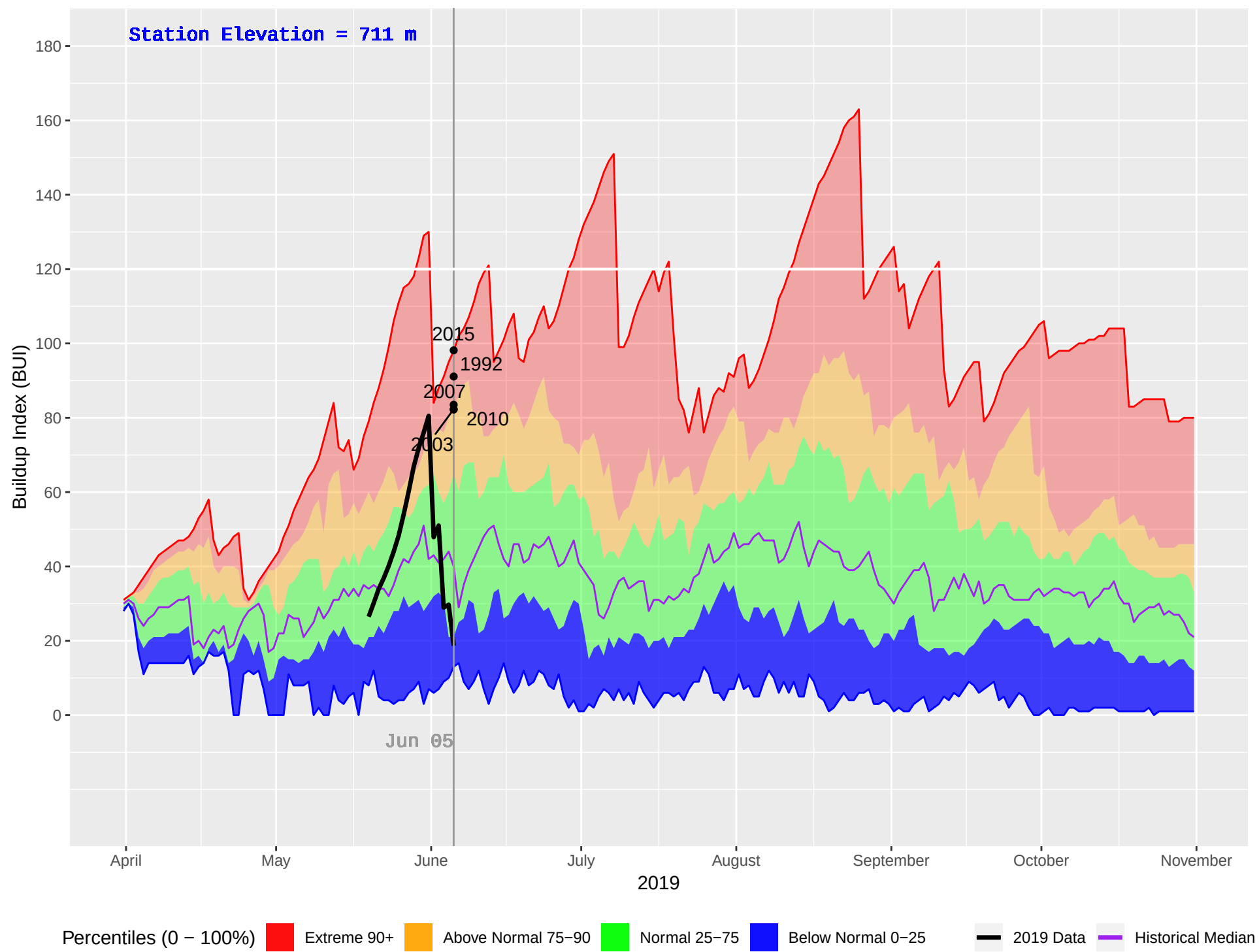
TOAD RIVER (126) : Historical (1981–2018), Current (2019) Daily Buildup Index (BUI)
