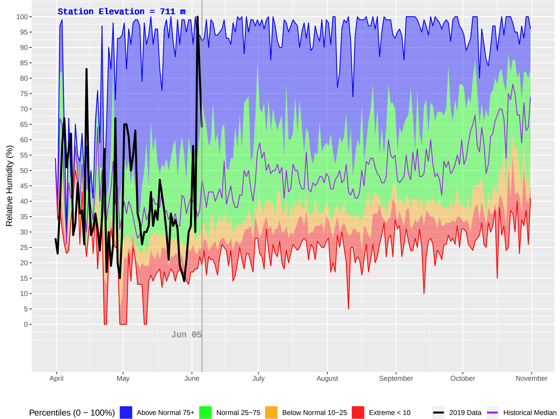
TOAD RIVER (126) : Historical (1981–2018) and Current (2019) Daily Relative Humidity
